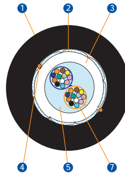
24 Fibre Construction
